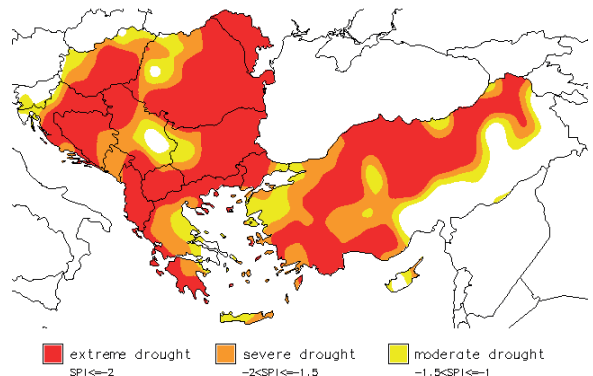
Figure 6. The SPI values presented for the month of April 2018, as output of “Drought Management Centre for Southeastern Europe” SPI Apr 2018 (1 month) GPCP first-guess analysis
