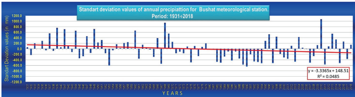
Figure 4. The standard deviation of rainfall values of Bushat meteorological station.
