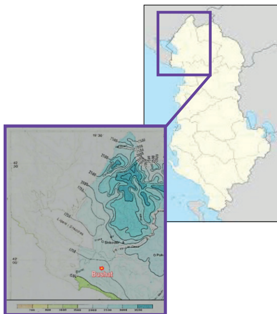
Figure 1. The Annual precipitation map of NW part of Lowland in Albania
