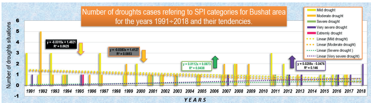
Figure 5. The tendency of different type of droughts for Bushat meteorological station standard
