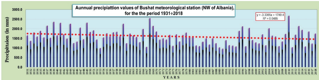
Figure 2. The annual precipitation values of Bushat meteorological station.
