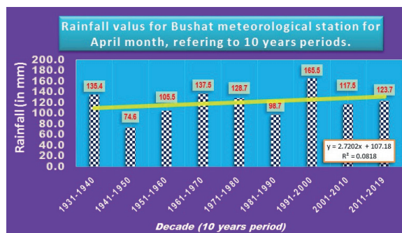
Figure 3. The 10 years period of rainfall for April month of Bushat meteorological station.
